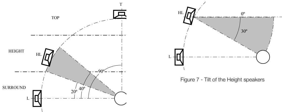
Figure 6 - Elevation angles
